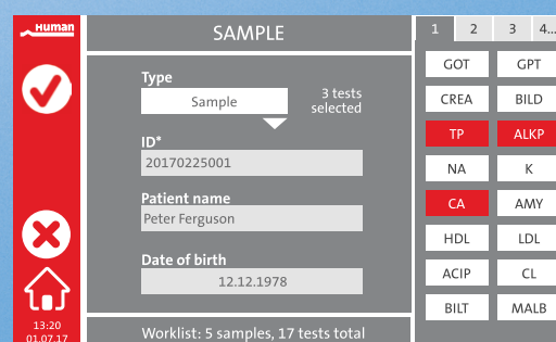
Sample Input
