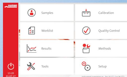
Main Menu
